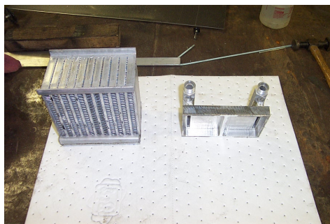
Milled heater core tank to withstand high pressuer of engine oil used as heat soure.
